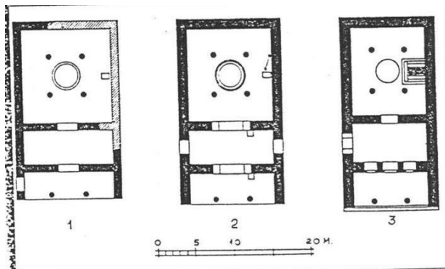
48. Ground plans of the Megara of Mycenae (1), Pylus (2) and Tiryns (3).
